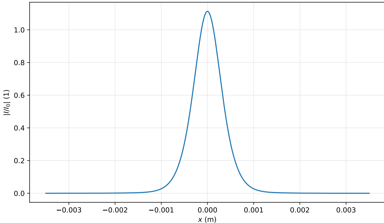
Intensity profile I(x, y = 0, z = 2.946m)/I_0 , P_{in}=0.8P_{cr} , artificial time
